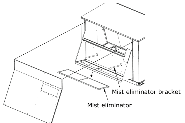
Figure 16. Mist eliminator removal
