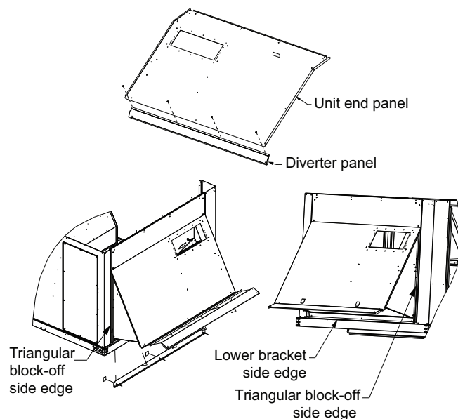
Figure 14. Rain diverter installation
