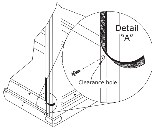
Figure 12. Remove gasket material
