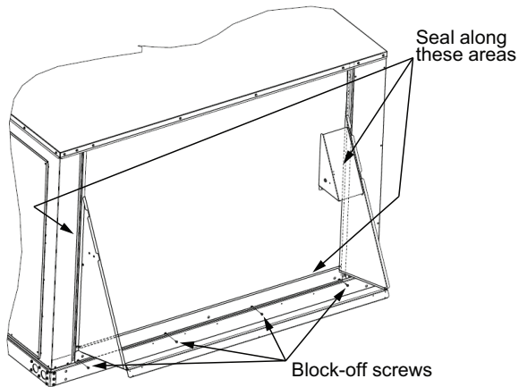
Figure 13. Block-off installation
