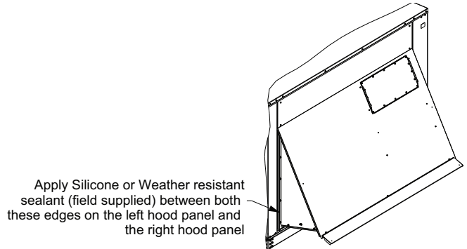
Figure 15. Sealant application location (both sides)
