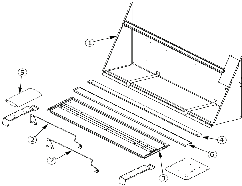
Figure 1. Major economizer components
