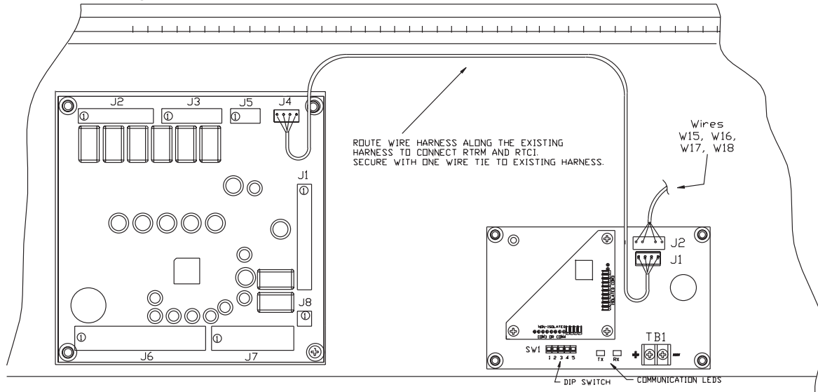
Figure 6 TCI Board Mounting and Wiring 6 - 10 Ton Packaged Rooftop units
