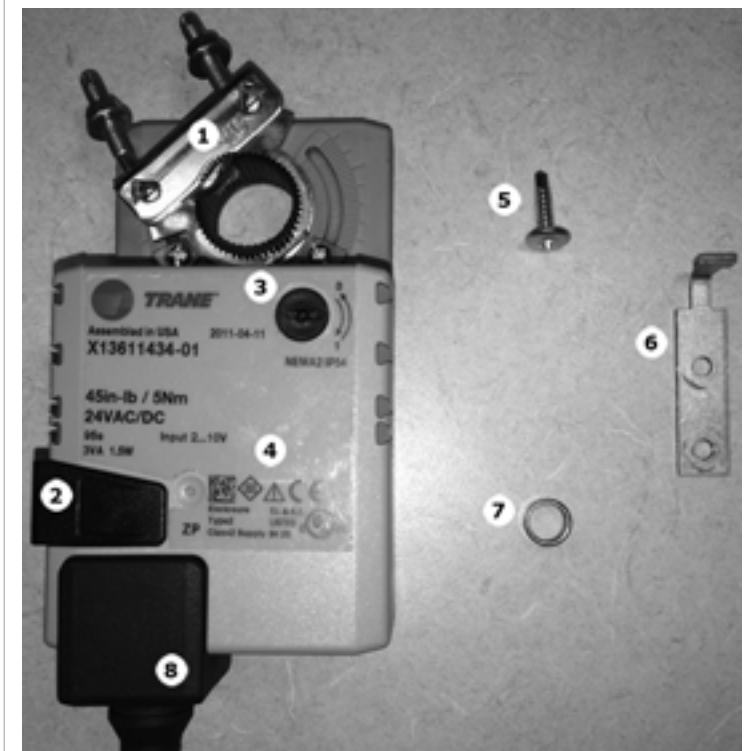
Figure 2. Trane actuator and parts
