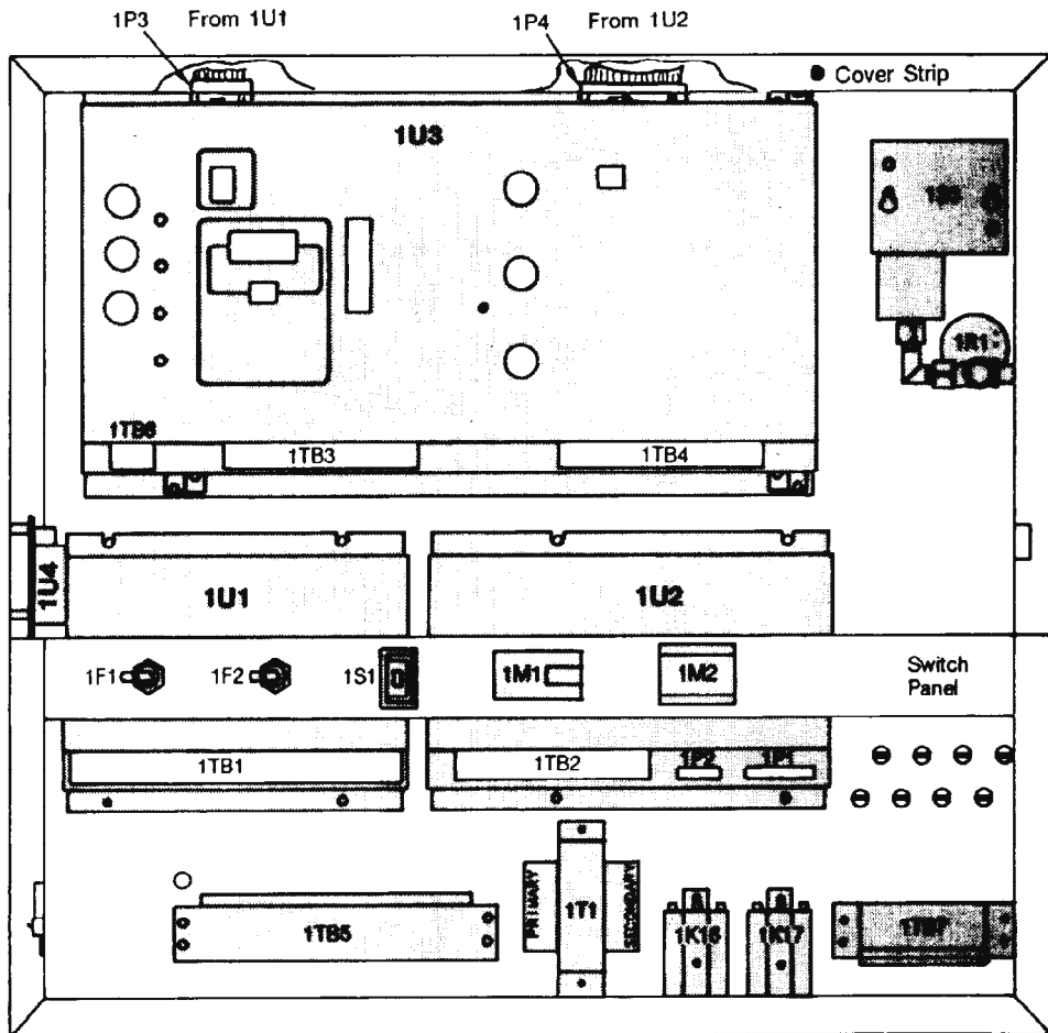
Figure 7 UCP Layout
