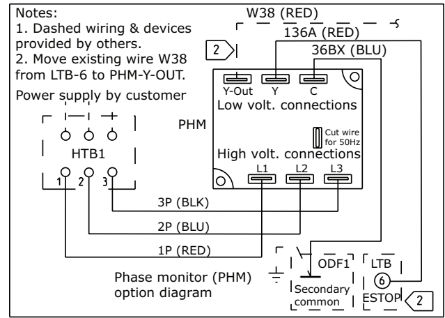
Figure 120. Phase monitor wiring diagram
