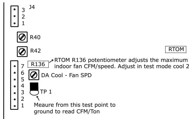
Figure 39. Adjusting airflow
