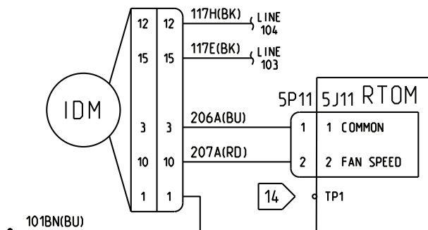
Figure 36. 17 Plus, 3 to 5 tons airflow control configuration
