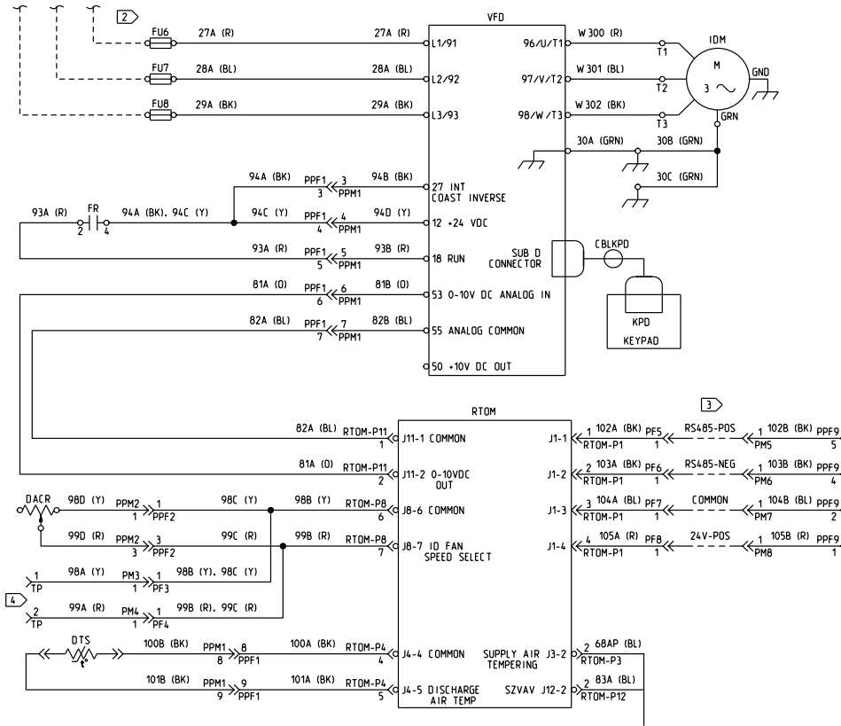
Figure 51. Odyssey™ RTOM
