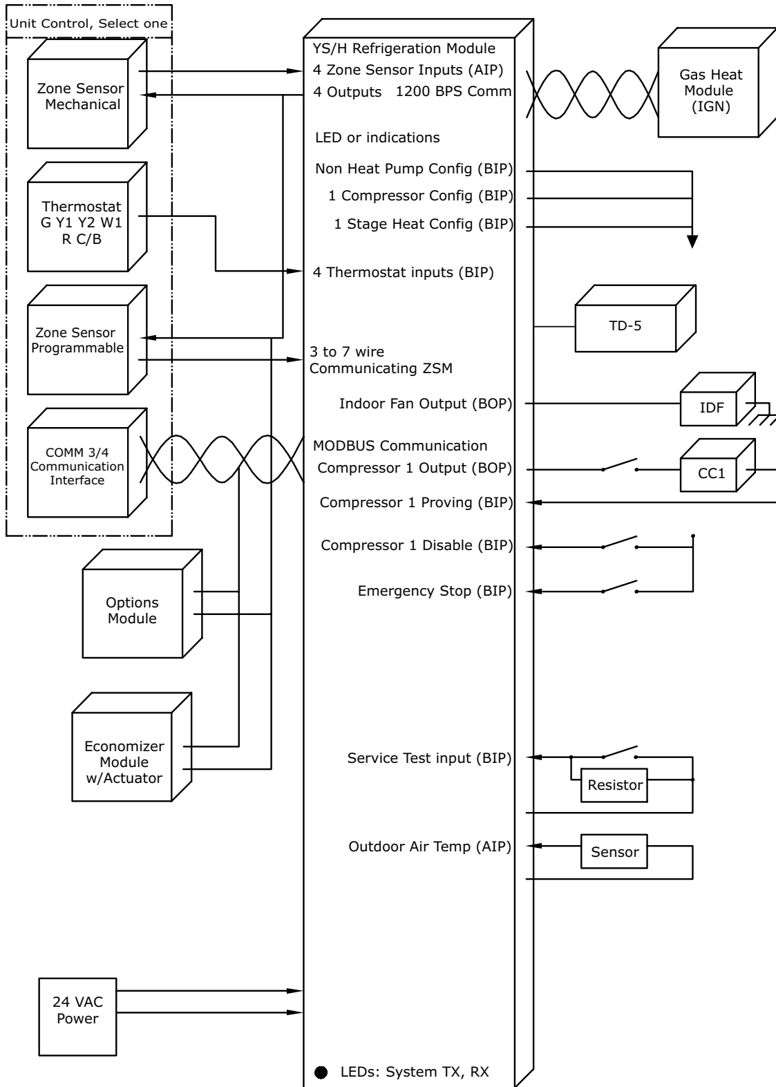
Figure 2. Precedent™ (YSC/YHC) refrigeration module (RTRM) gas heating
