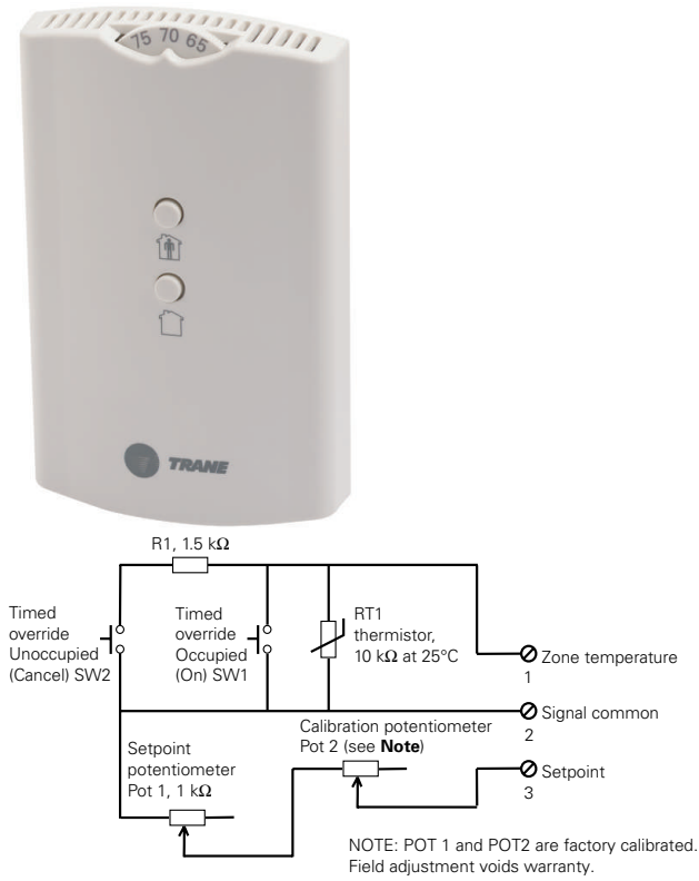
Figure 65. BAYSENS074*
