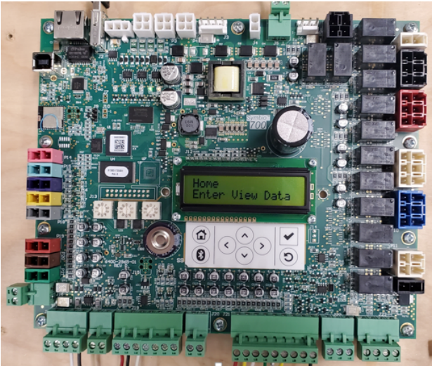
Figure 4. Symbio 700 controller
