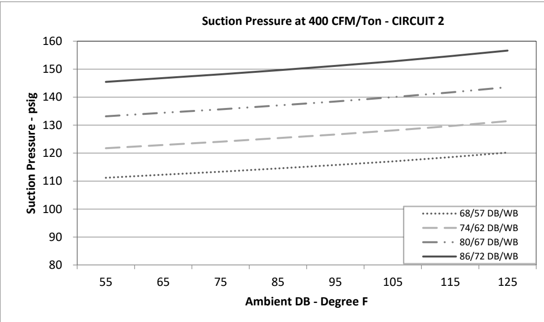
Circuit 2
