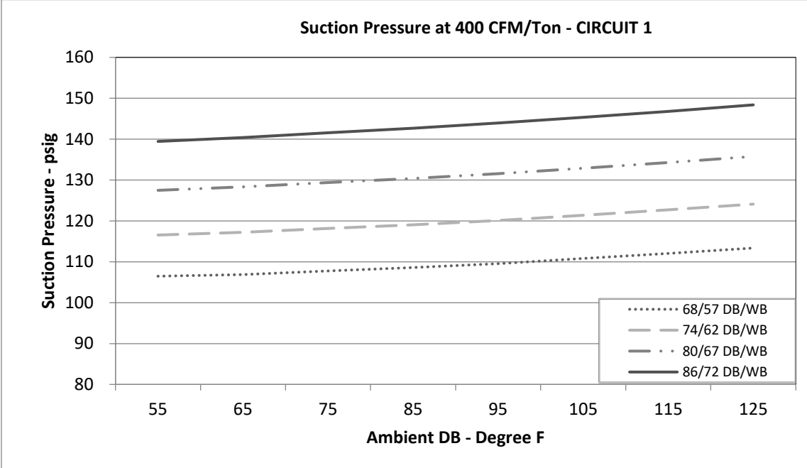
Circuit 1
