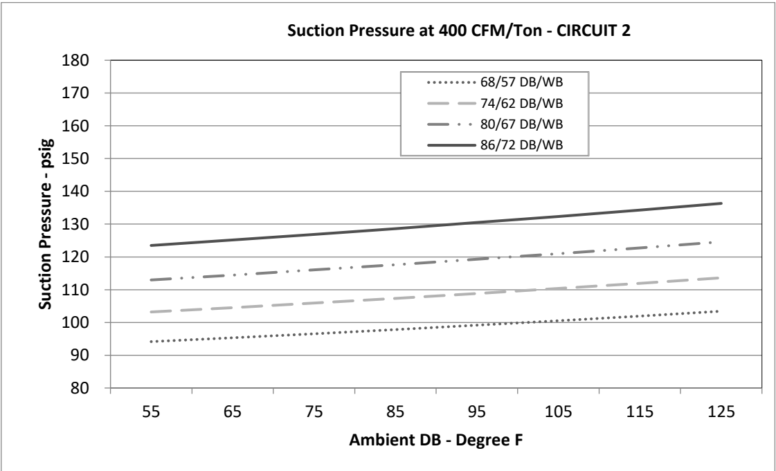
Circuit 2
