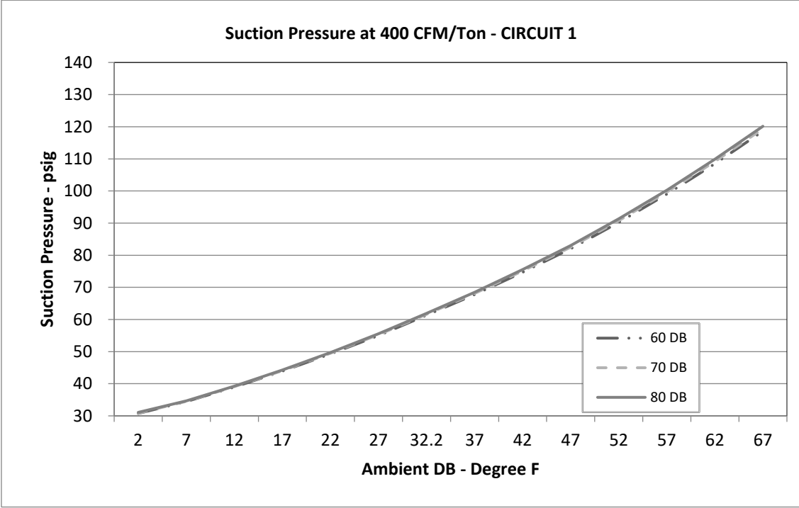
Circuit 1
