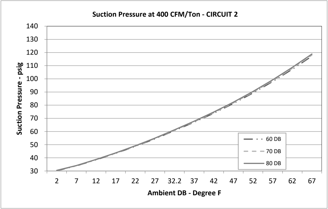
Circuit 2
