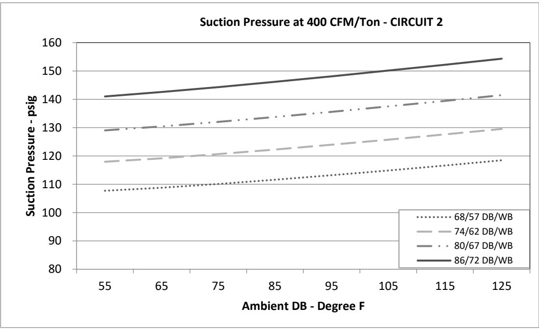
Circuit 2
