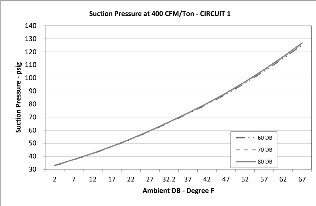
Circuit 1
