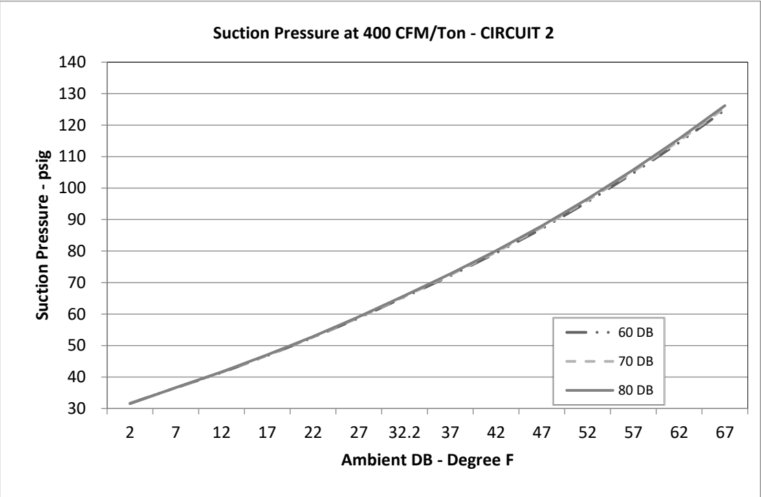
Circuit 2
