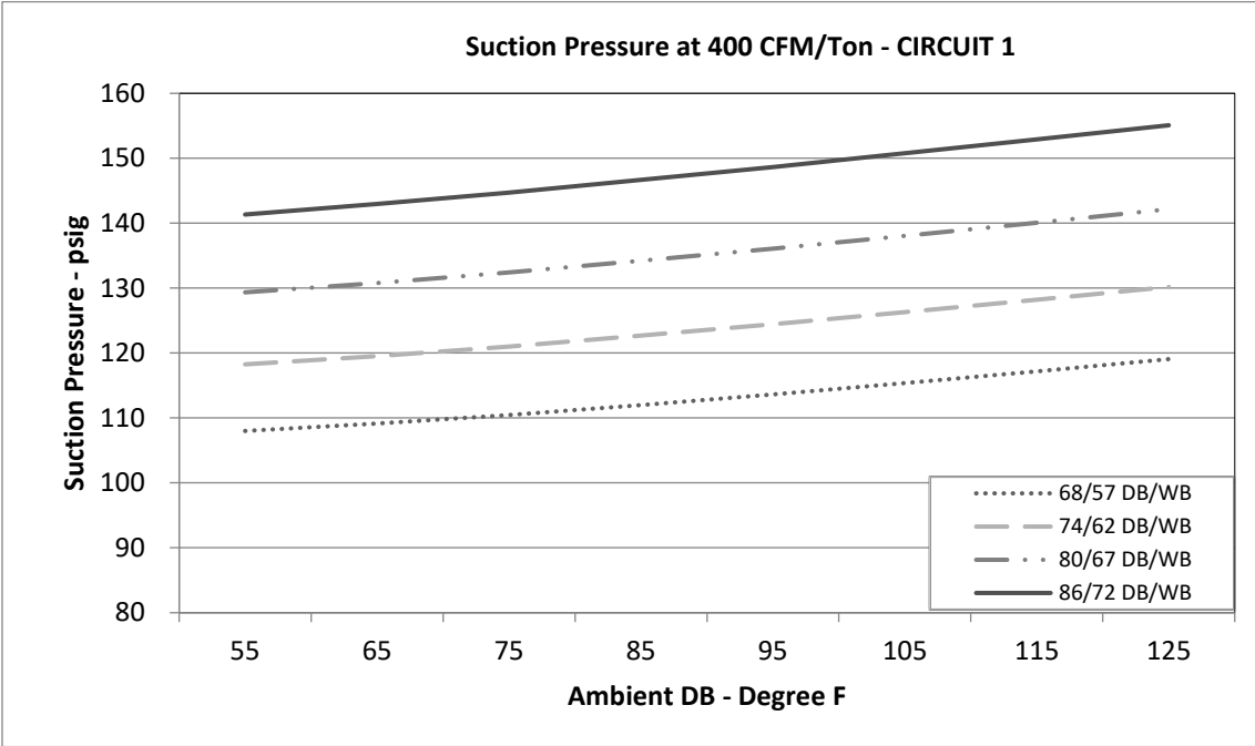
Circuit 1
