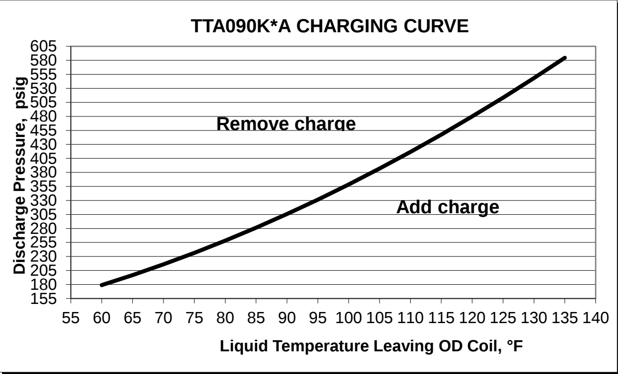
Pressure curve TTA090K*A with TWE090K*A:
