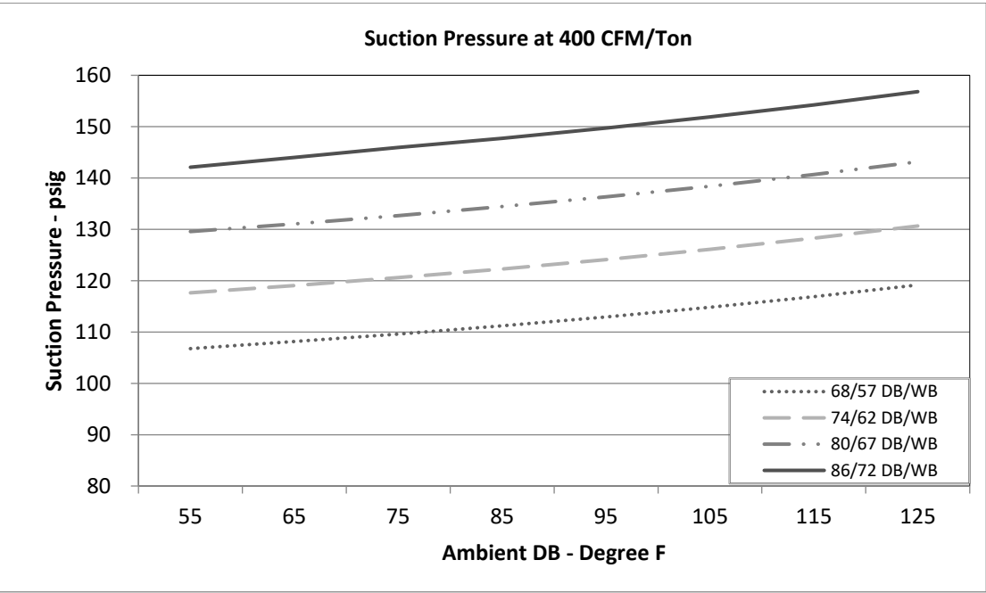
Pressure curve TTA090K*A with TWE090K*A:
