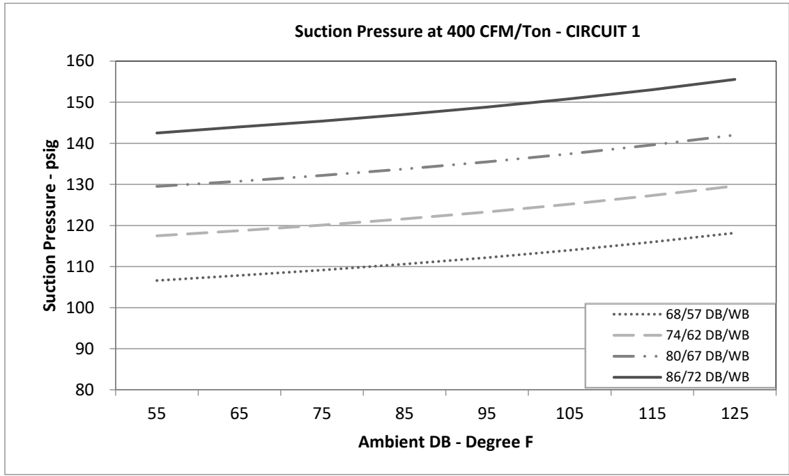
Circuit 1
