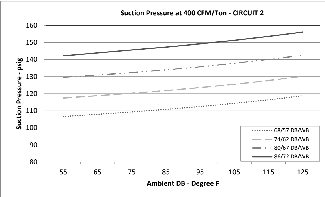
Circuit 2
