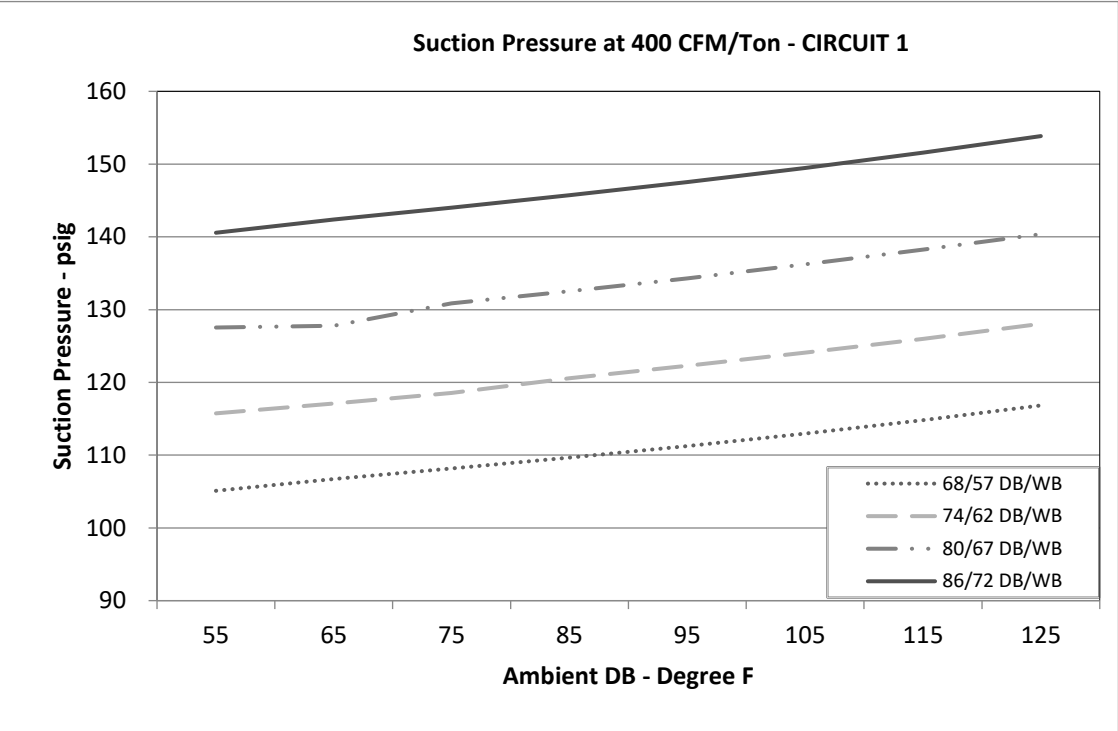
Circuit 1
