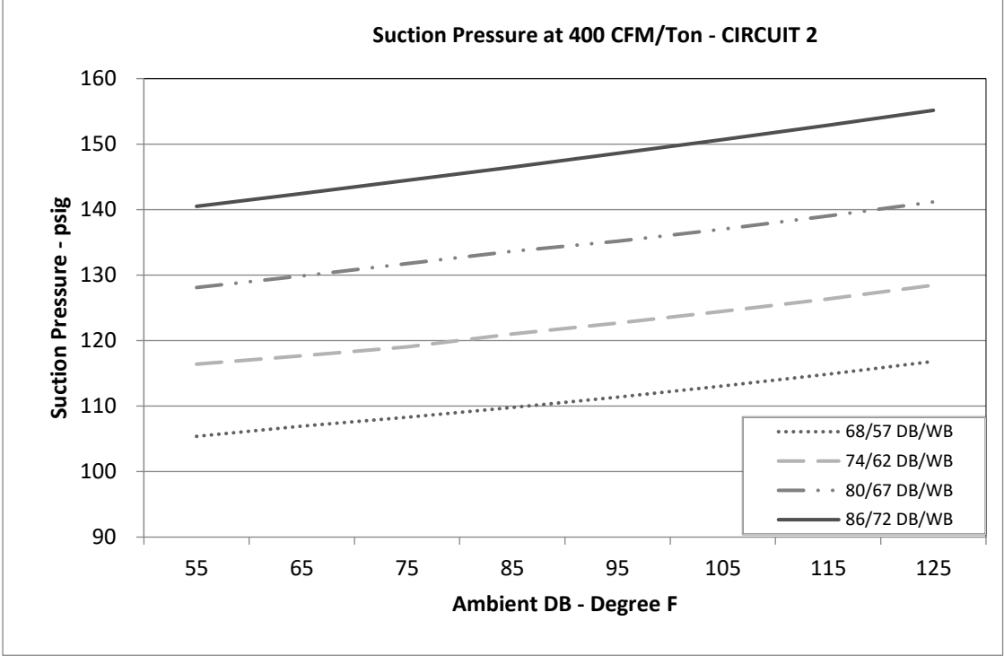
Circuit 2
