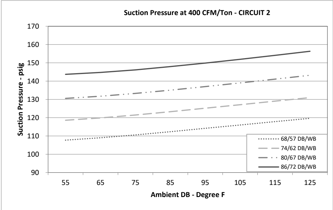
Circuit 2
