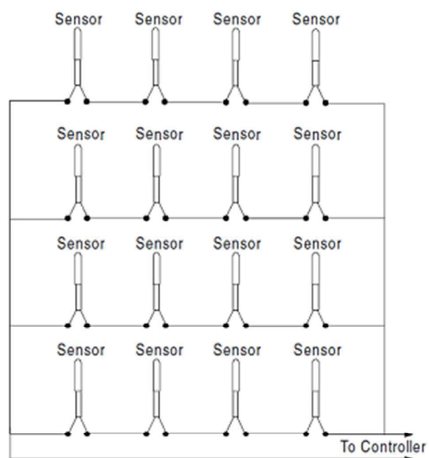
Figure 4: 16-Sensor Averaging Wiring
