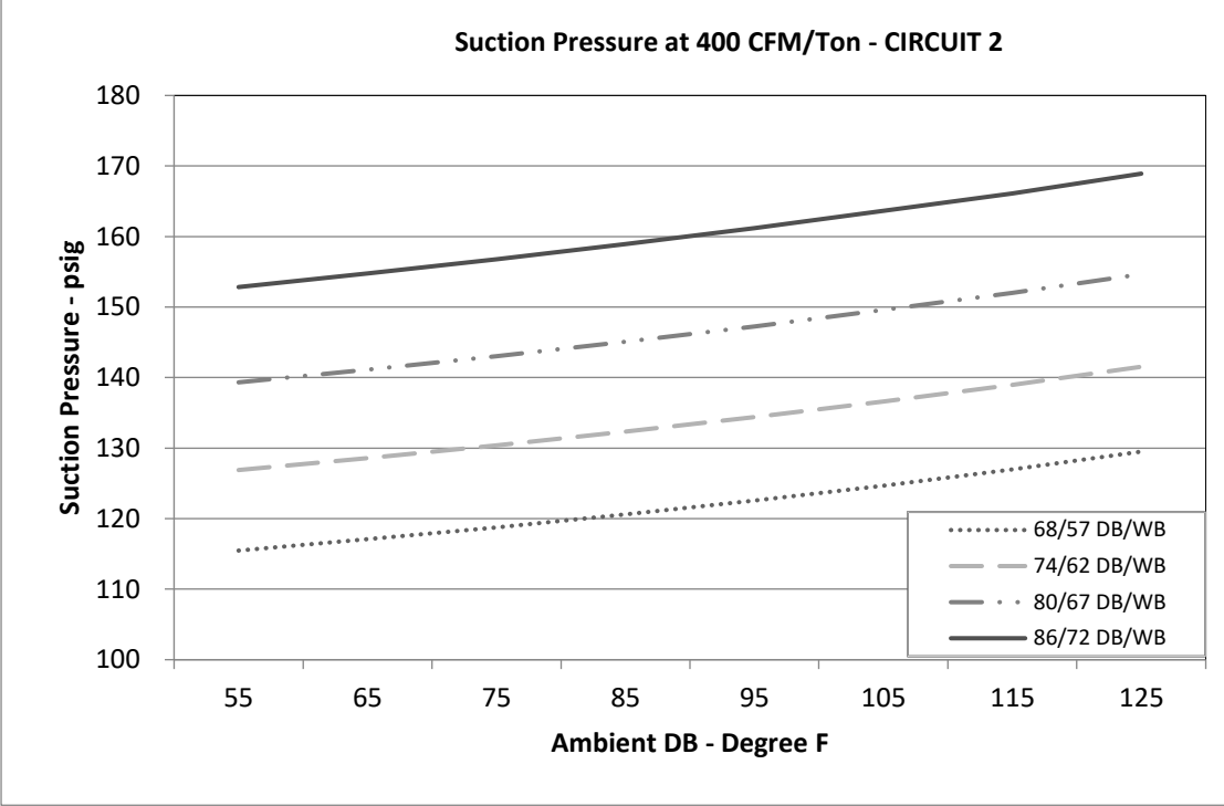
Circuit 2
