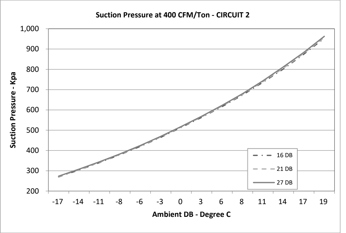
Circuit 2
