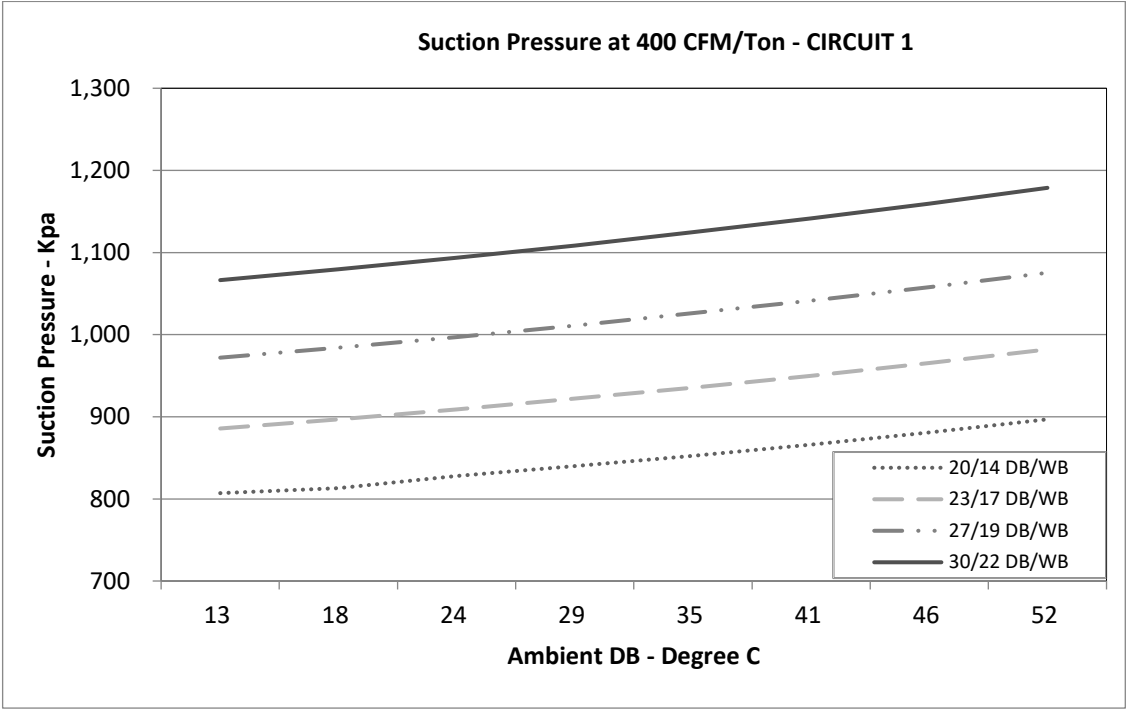
Circuit 1
