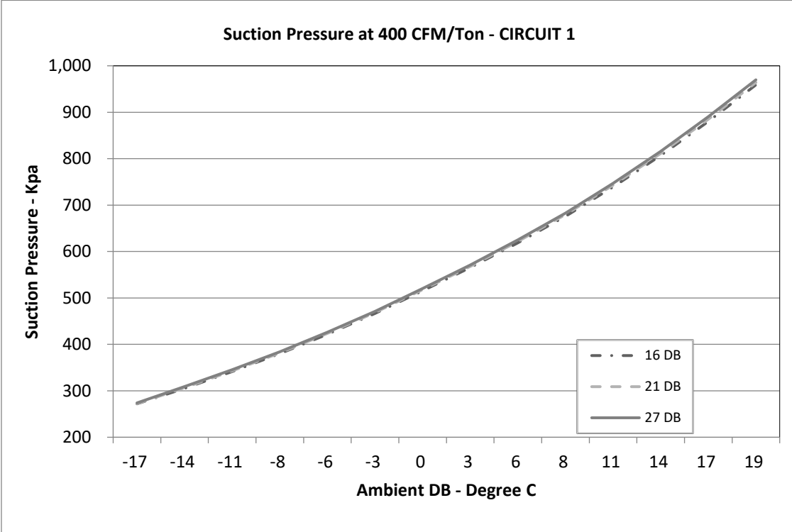
Circuit 1
