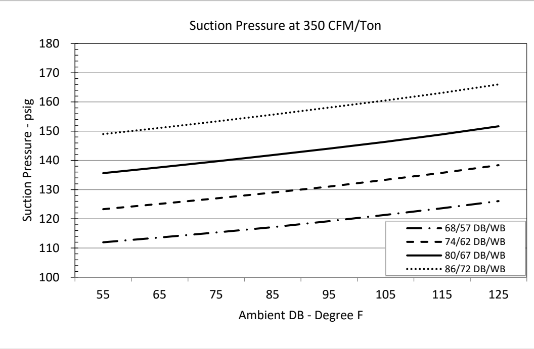
Circuit 1
