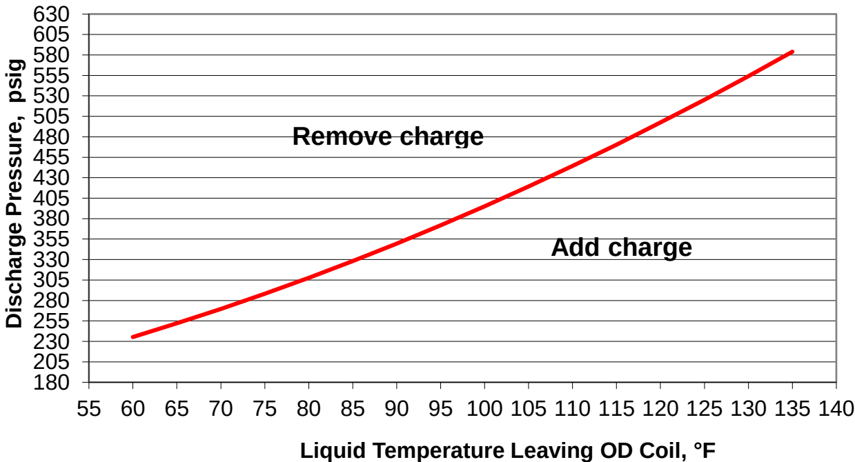
Both Compressors Running TWA0904*D CHARGING CURVE - COOLING MODE
