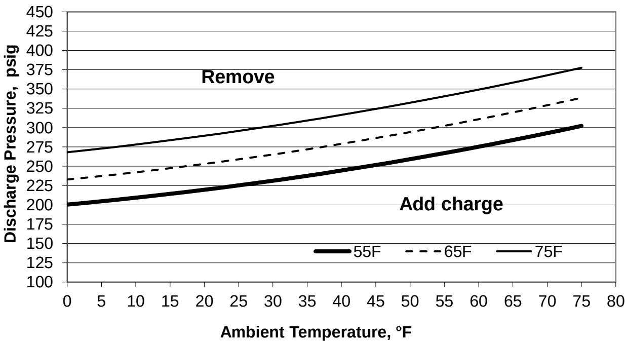
Both Compressors Running TWA0904*D CHARGING CURVE - HEATING MODE
