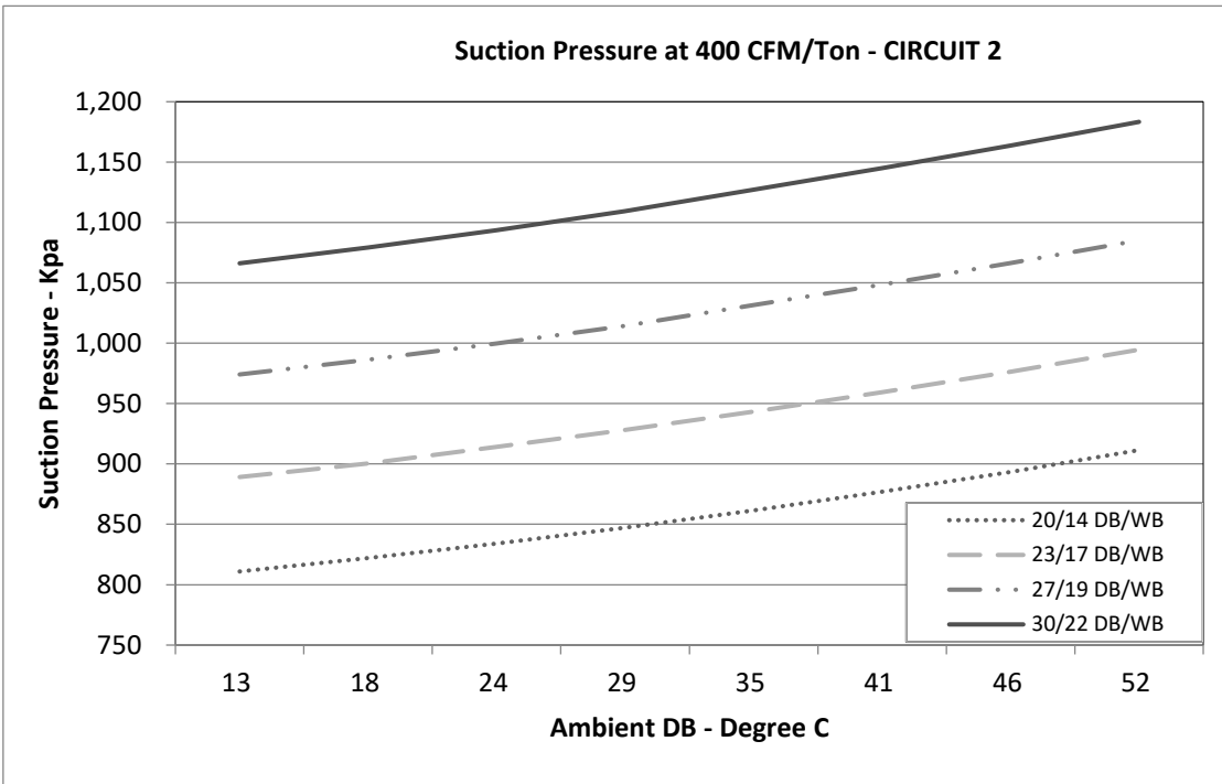
Circuit 2
