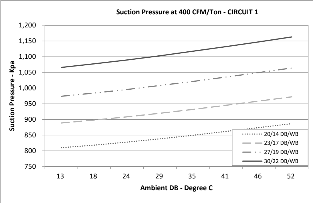
Circuit 1
