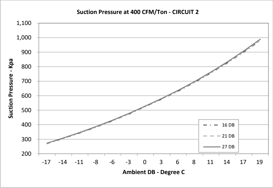
Circuit 2
