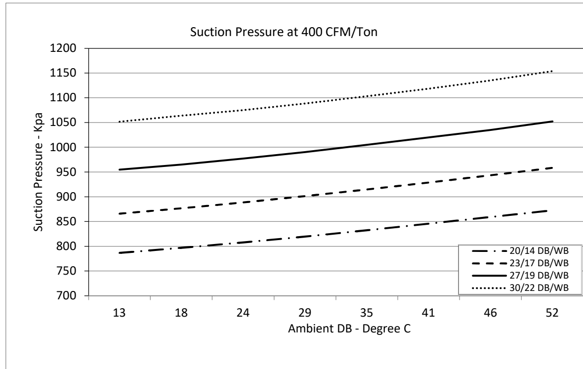
Pressure curve TTA0764DA with TWE0764DA:
