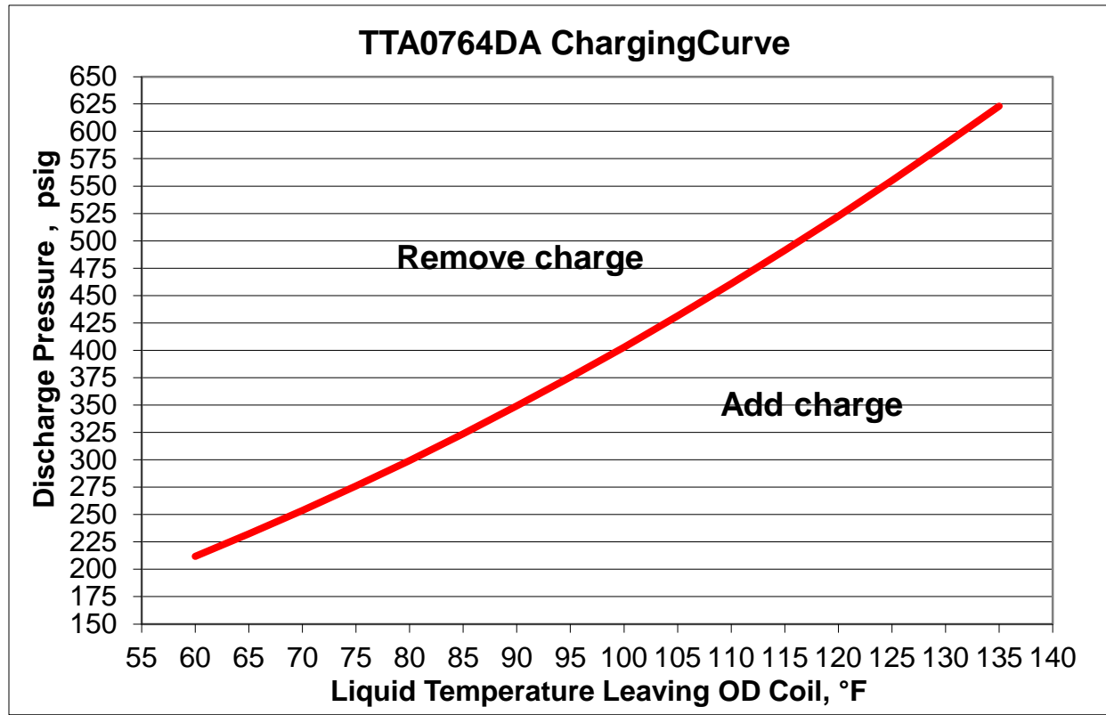
Pressure curve TTA0764DA with TWE0764DA:
