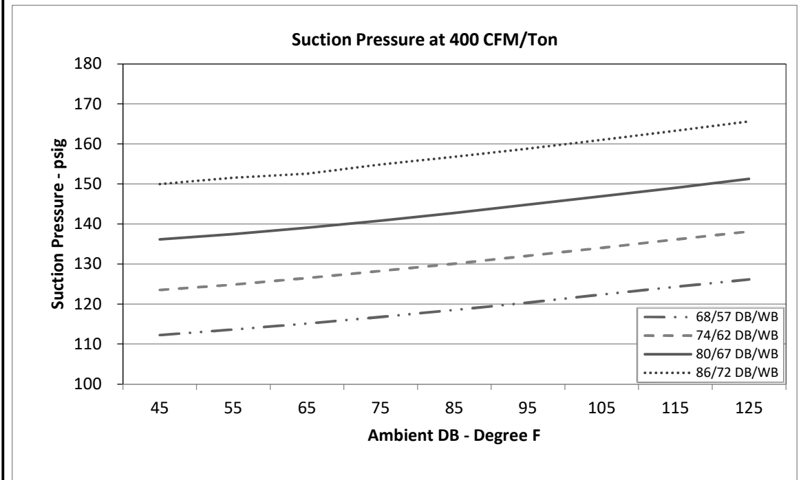
Circuit 2
