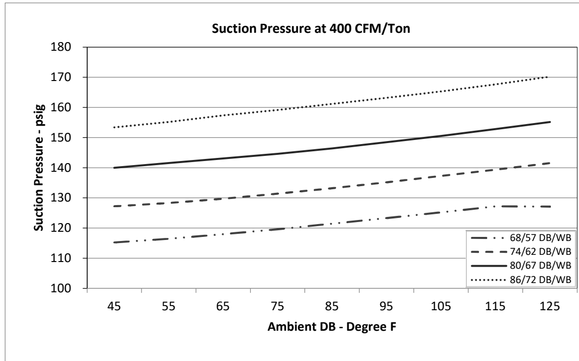
Circuit 1
