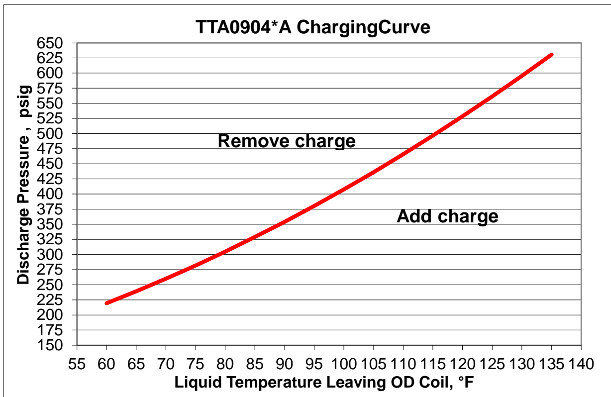
Pressure curve TTA0904*A with TWE0904*A:
