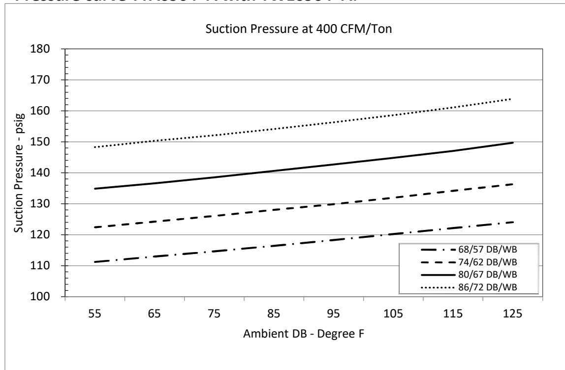
Pressure curve TTA0904*A with TWE0904*A:
