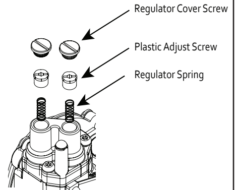
Fig. 4 Gas Valve
